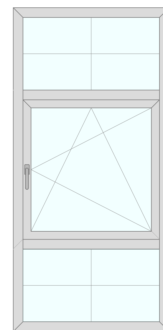
FIXED OPERABLE TILT & TURN, AND FIXED WINDOW
