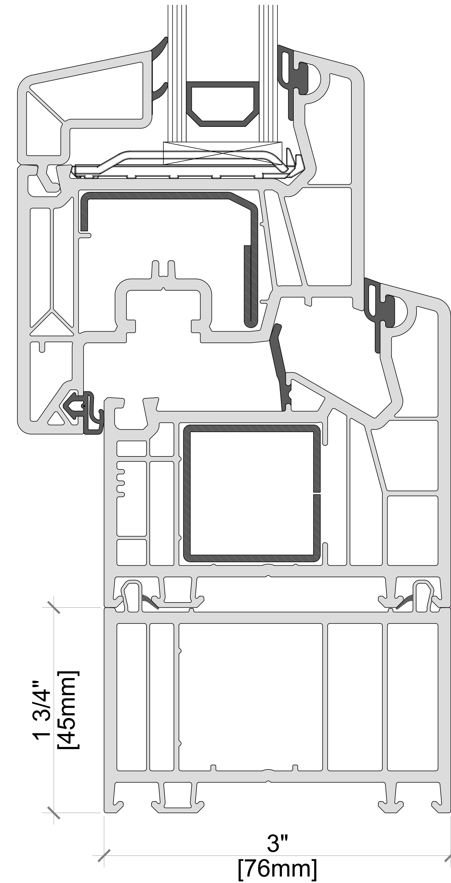
45mm SUB SILL: 114054 SUB SILL 45mm
