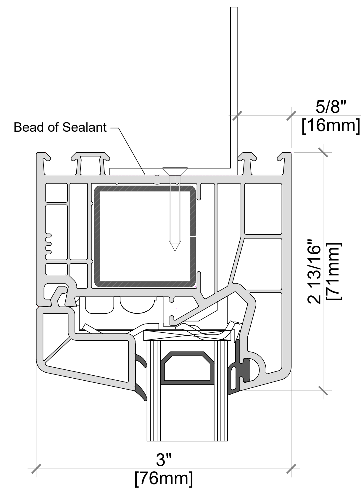
76mm FIXED PROFILE WITH ALU FLANGE
