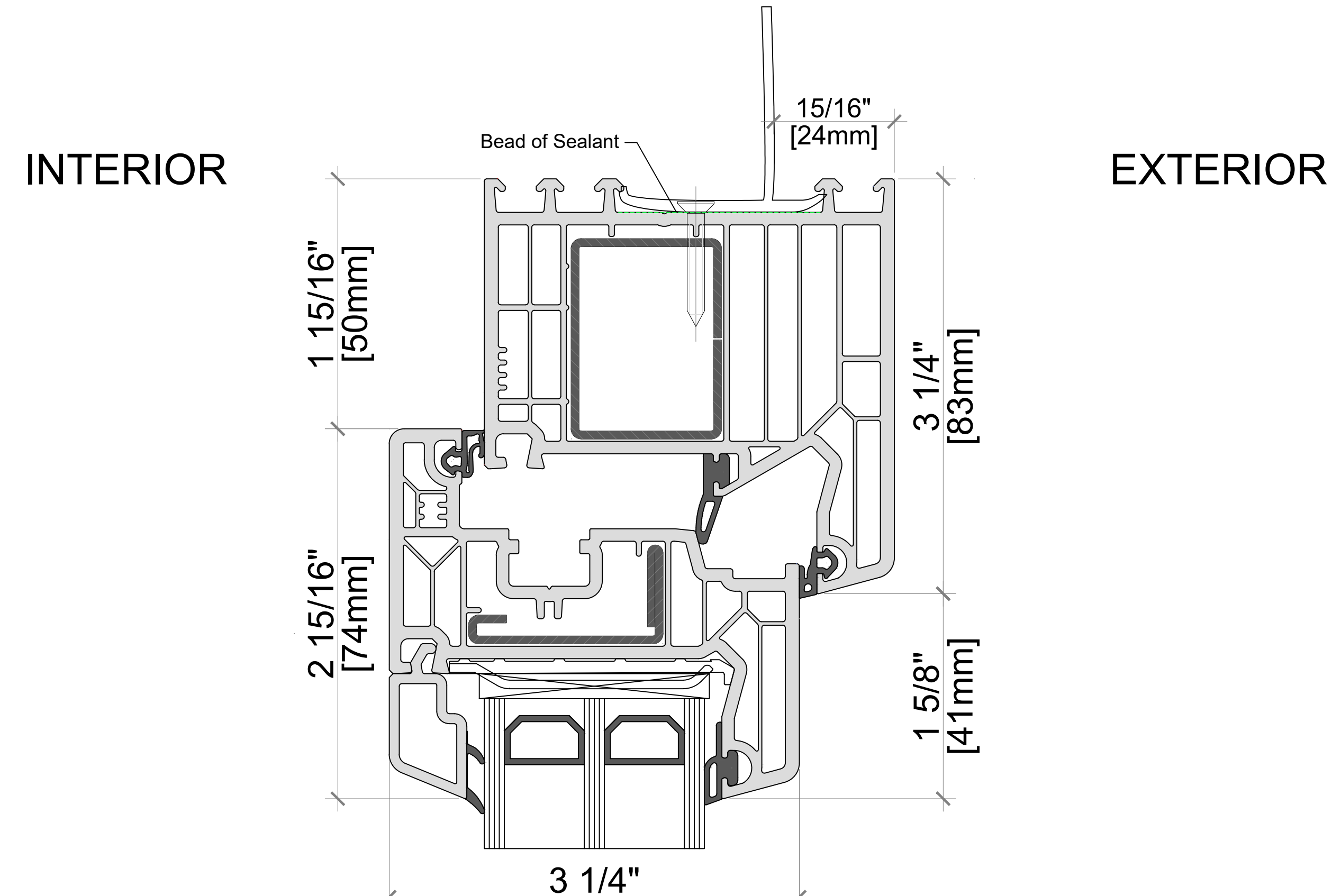
82mm OPERABLE WINDOW WITH PVC FLANGE
