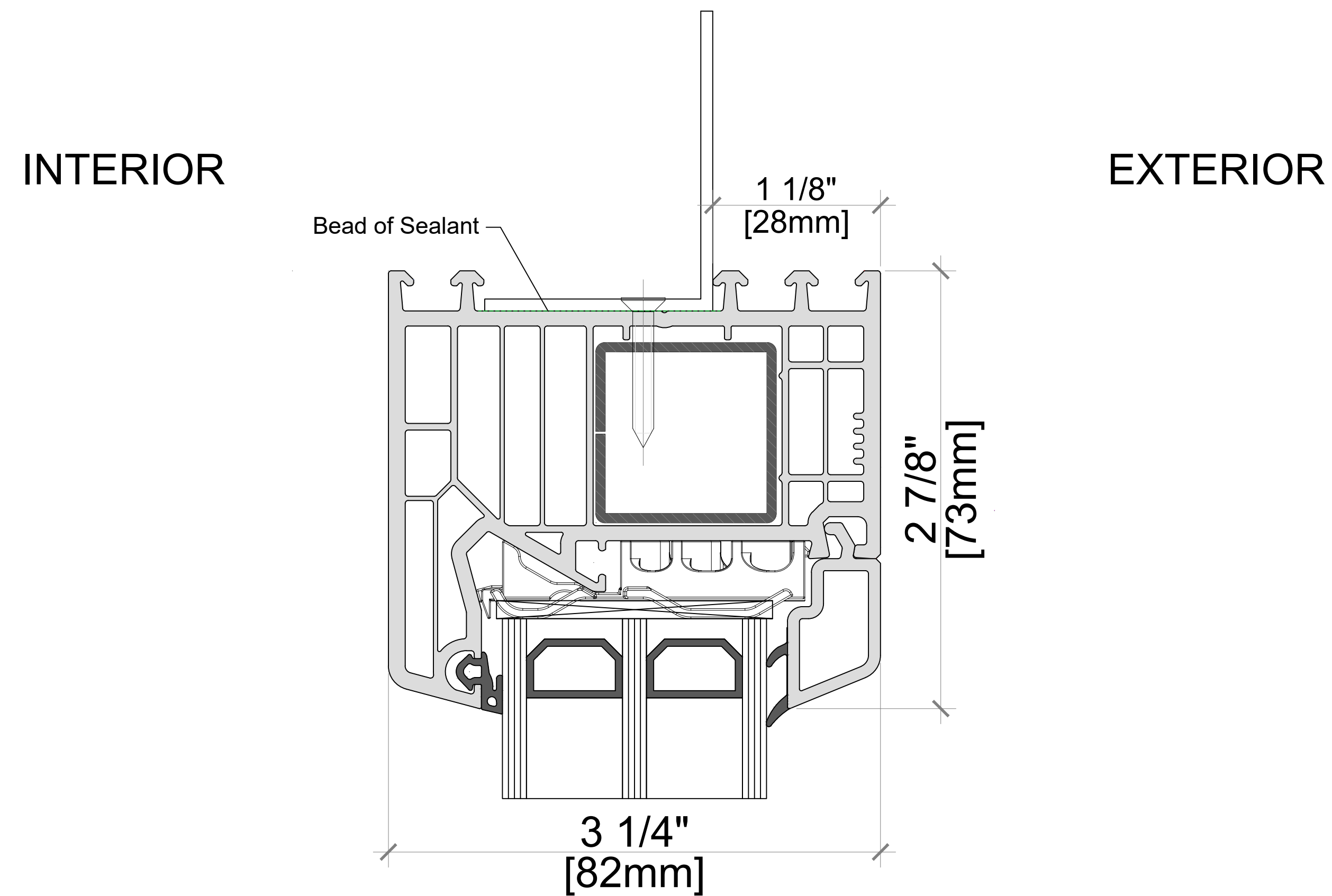
82mm FIXED PROFILE WITH ALU FLANGE
