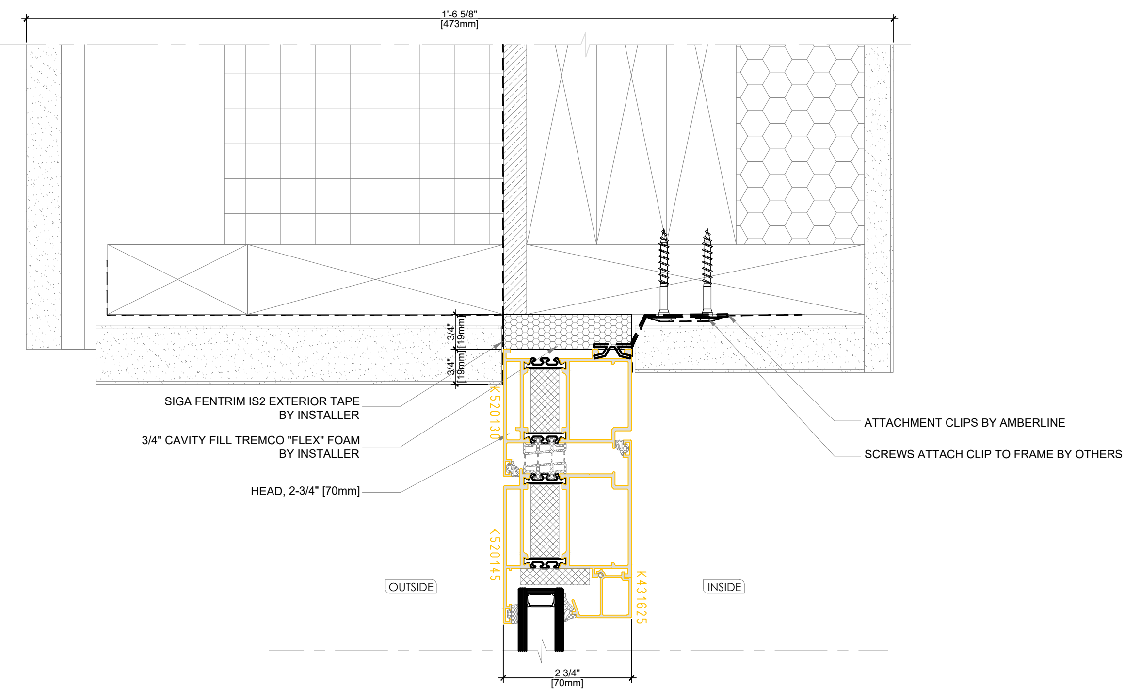
1 ENTRY DOOR HEAD DETAIL DG-ALU79 -2 SCALE: 1:2
