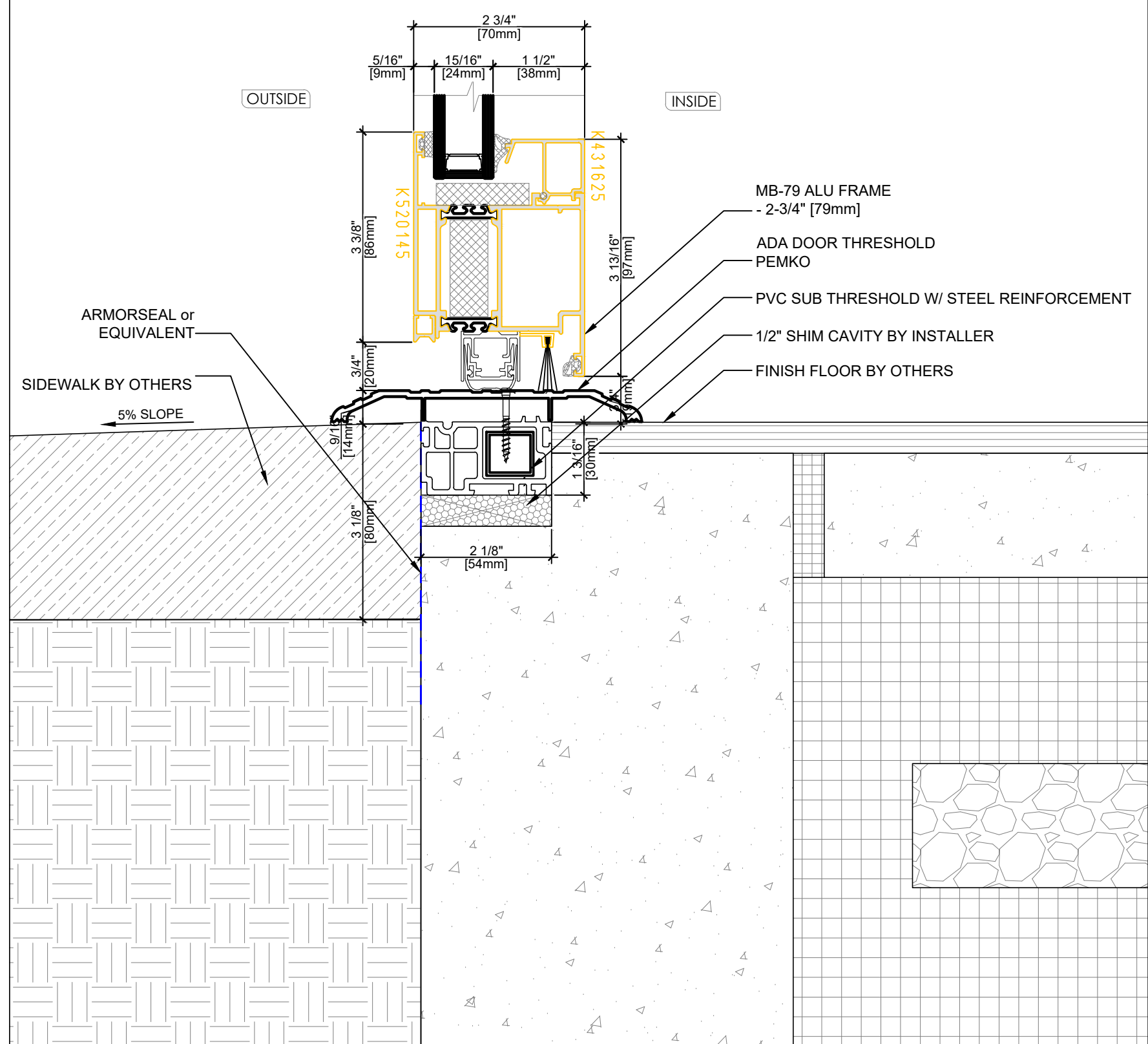
2A Option A: ADA ENTRY DOOR SILL DETAIL DG-ALU79-1 SCALE: 1:2 Complies with MA CMR 521
