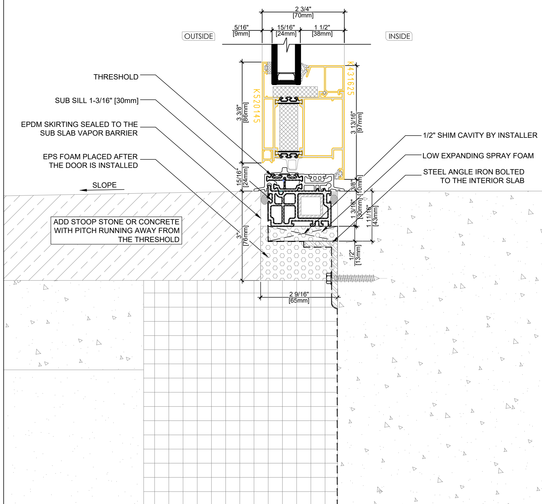
2B Option B: ENTRY DOOR SILL DETAIL DG-ALU79 -2 SCALE: 1:2
