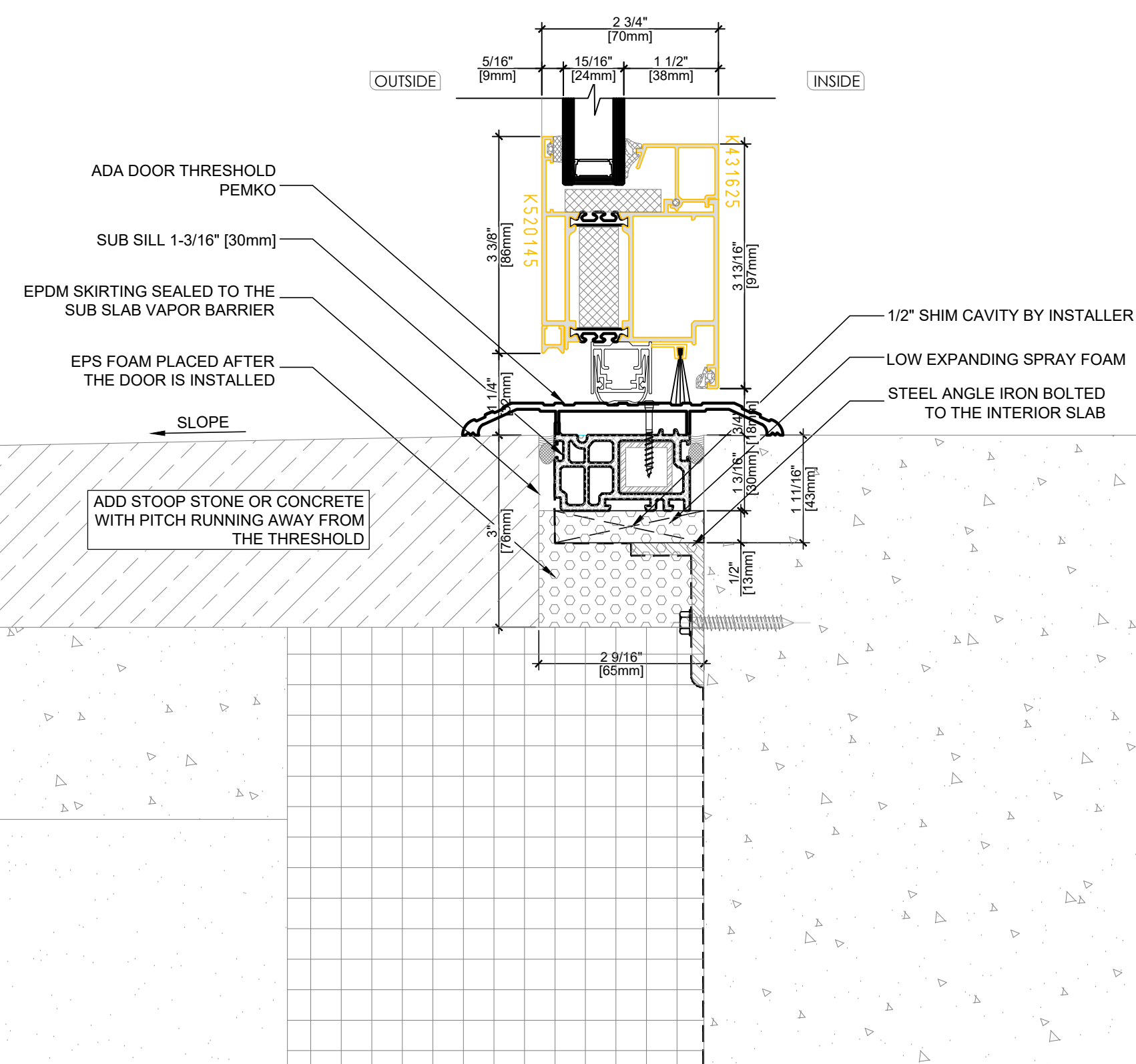
2A Option A: ADA ENTRY DOOR SILL DETAIL DG-ALU79 -2 SCALE: 1:2 Complies with MA CMR 521
