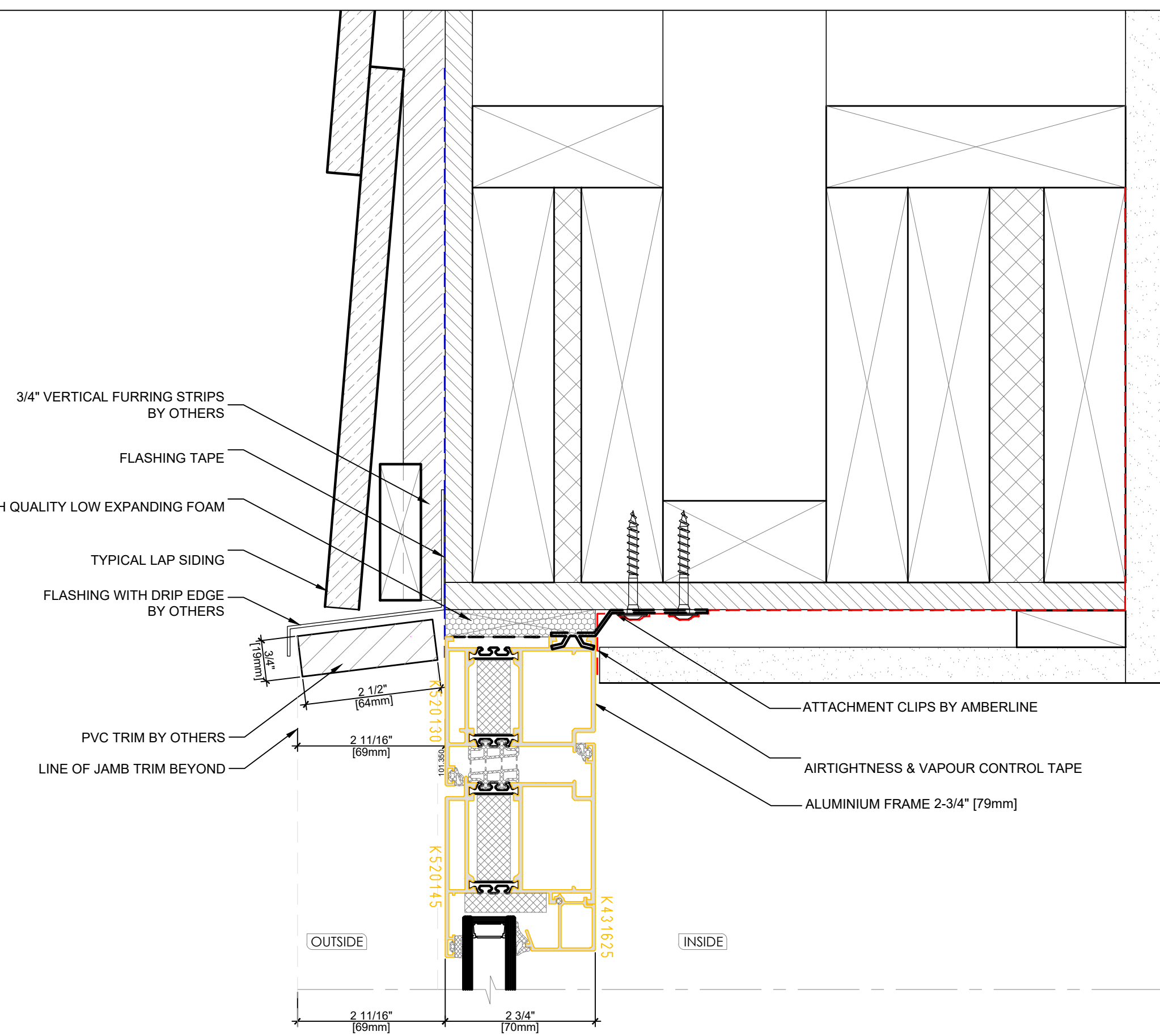
1 ENTRY DOOR HEAD DETAIL DG-ALU79-1 SCALE: 1:2
