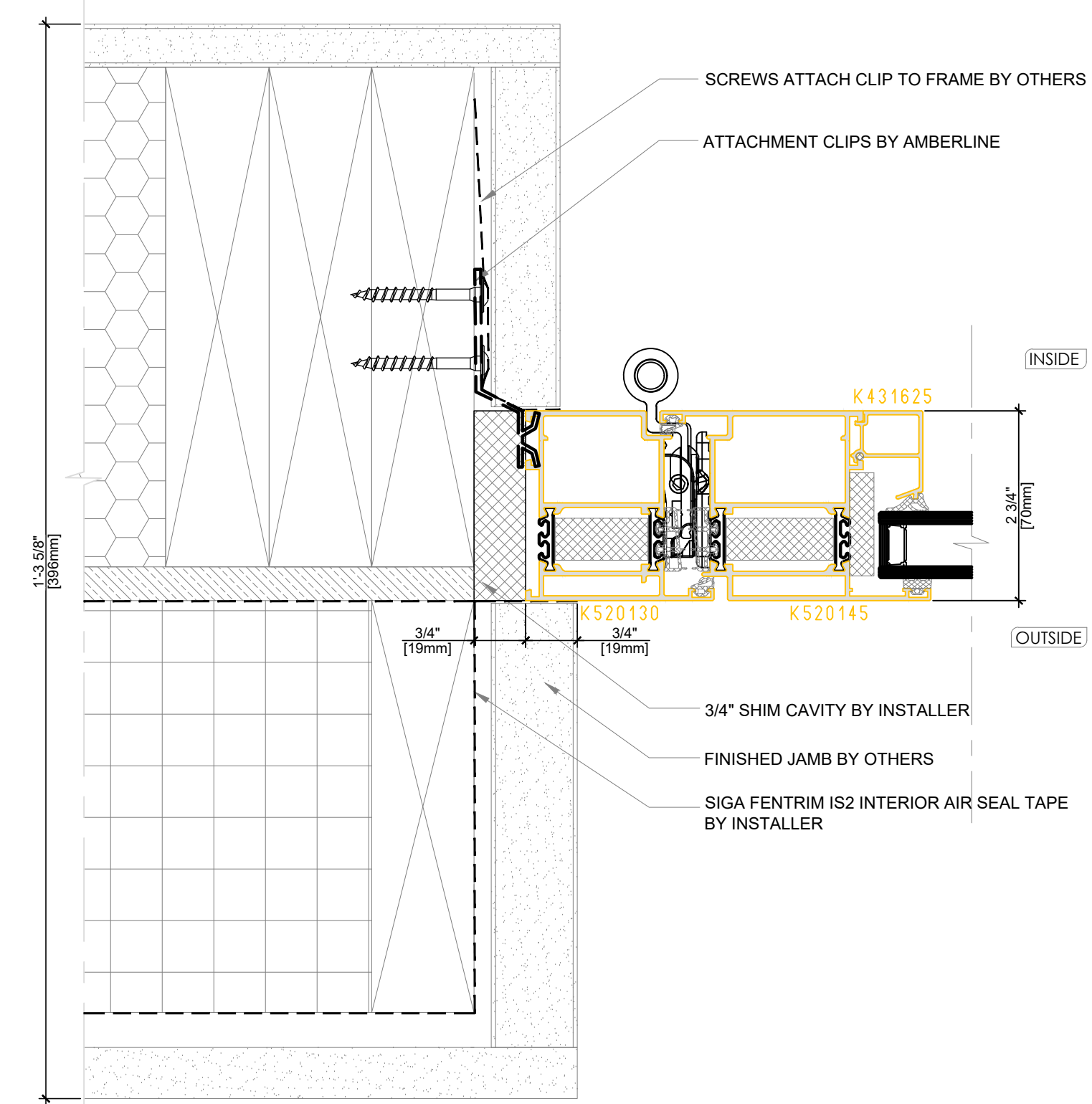
3 ENTRY DOOR JAMB DETAIL DG-ALU79 -2 SCALE: 1:2
